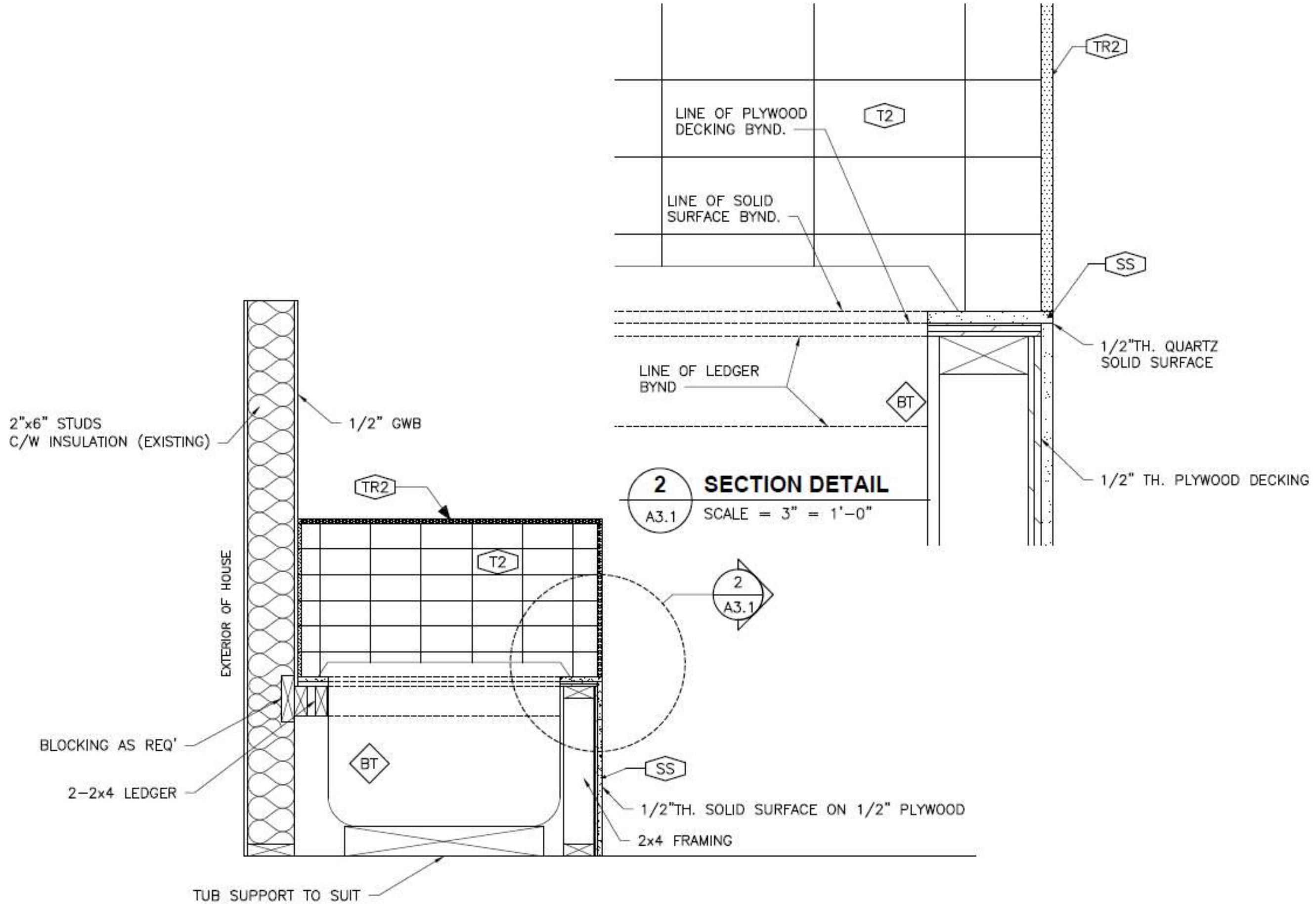
1 BATH SECTION A3.1 SCALE = 1" = 1'-0"
