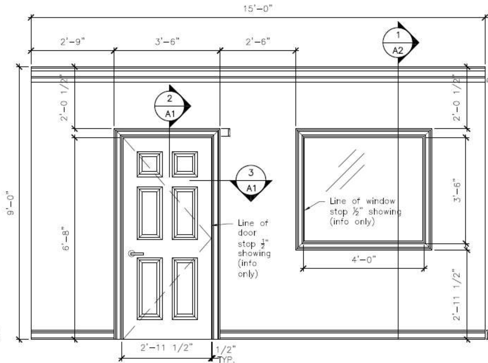
1 INTERIOR WALL ELEVATION A1 SCALE: 1/2"=1'-0"
