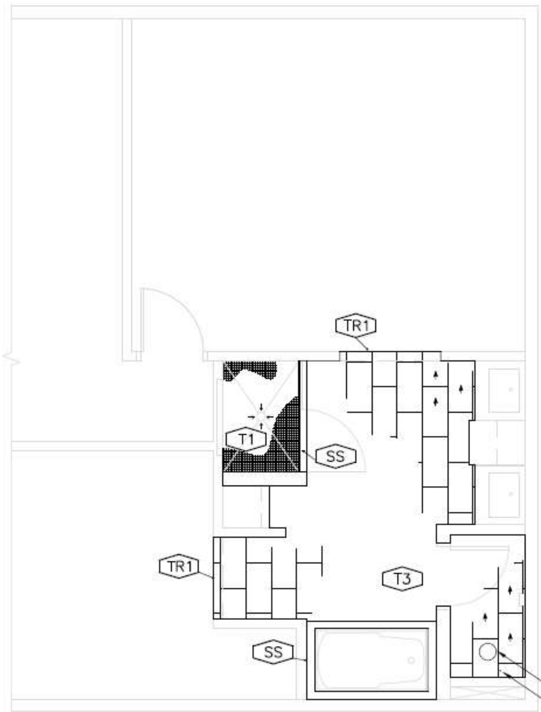
1 FINISH PLAN A1.2 SCALE = 1/4" = 1' - 0"
