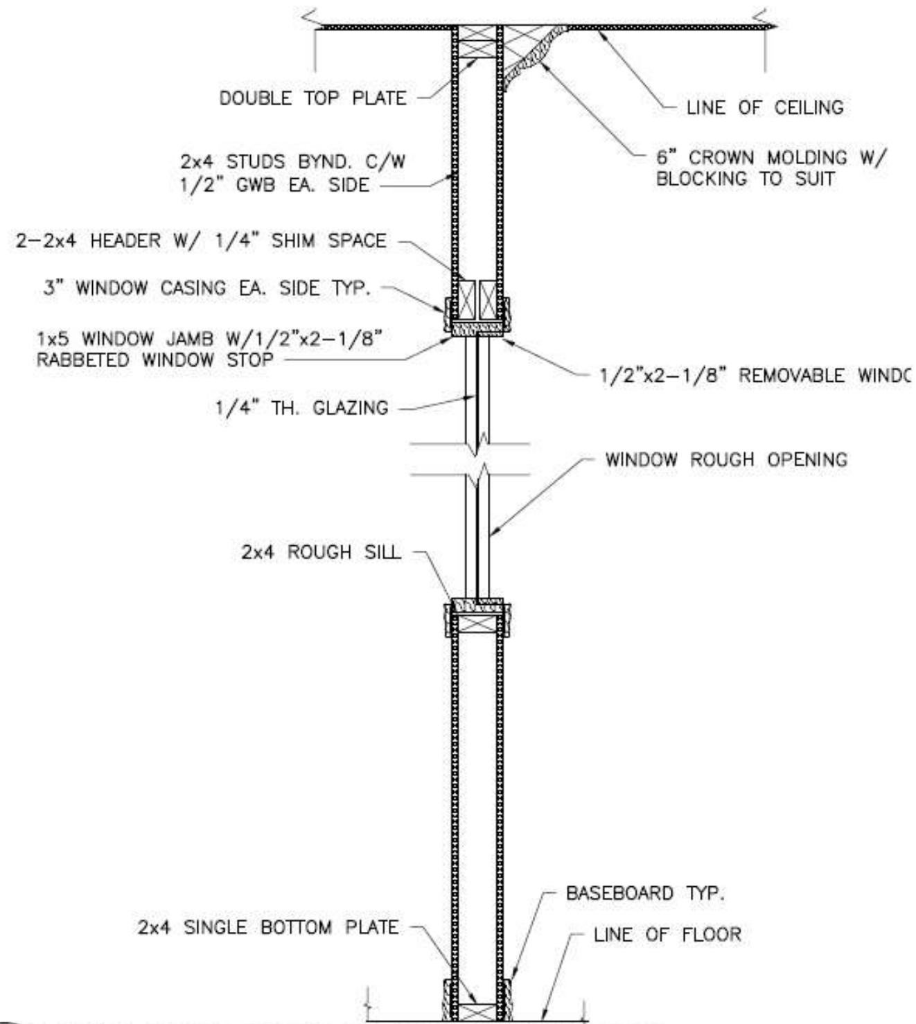
4 FULL WALL SECTION THROUGH WINDOW A2 SCALE: 1"=1'-0"
